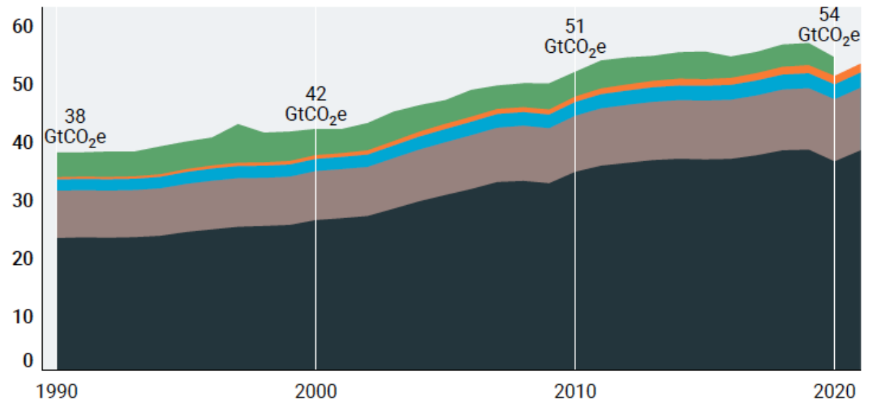
Total GHG emissions 1990–2021 (GtCO 2 e/year)
